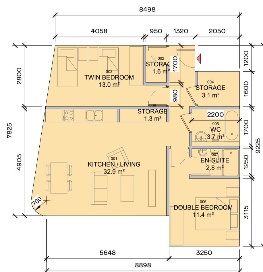
73.2 m 2 4 APARTMENT TYPE - 2B-5B 1:100
