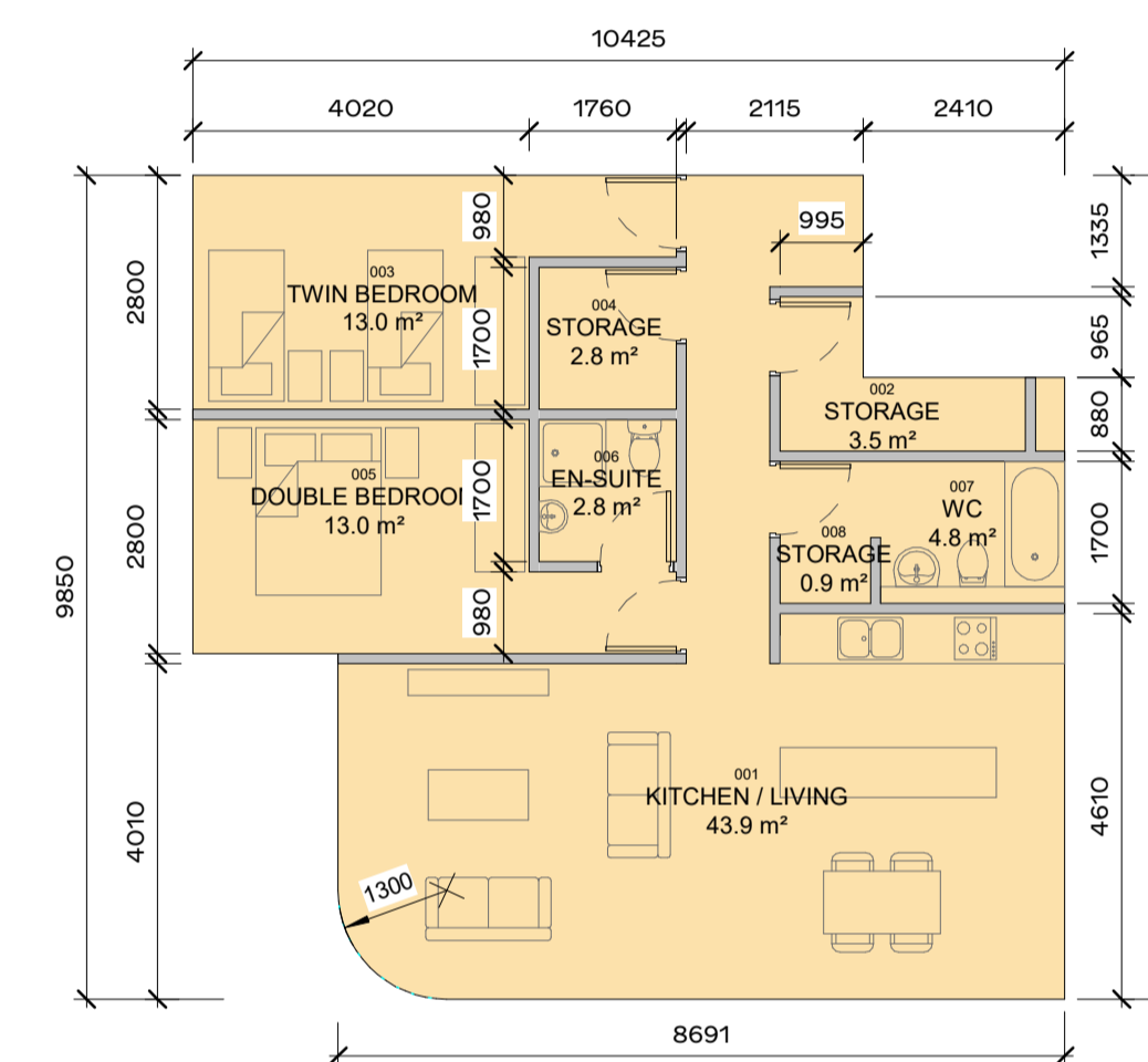
89.3 m 2 7 APARTMENT TYPE - 2B-6B 1:100
