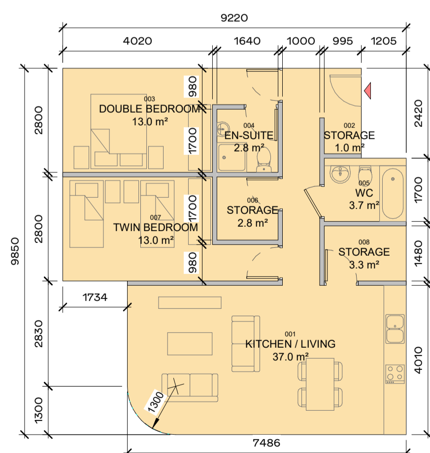
80.4 m 2 5 APARTMENT TYPE - 2B-6A 1:100
