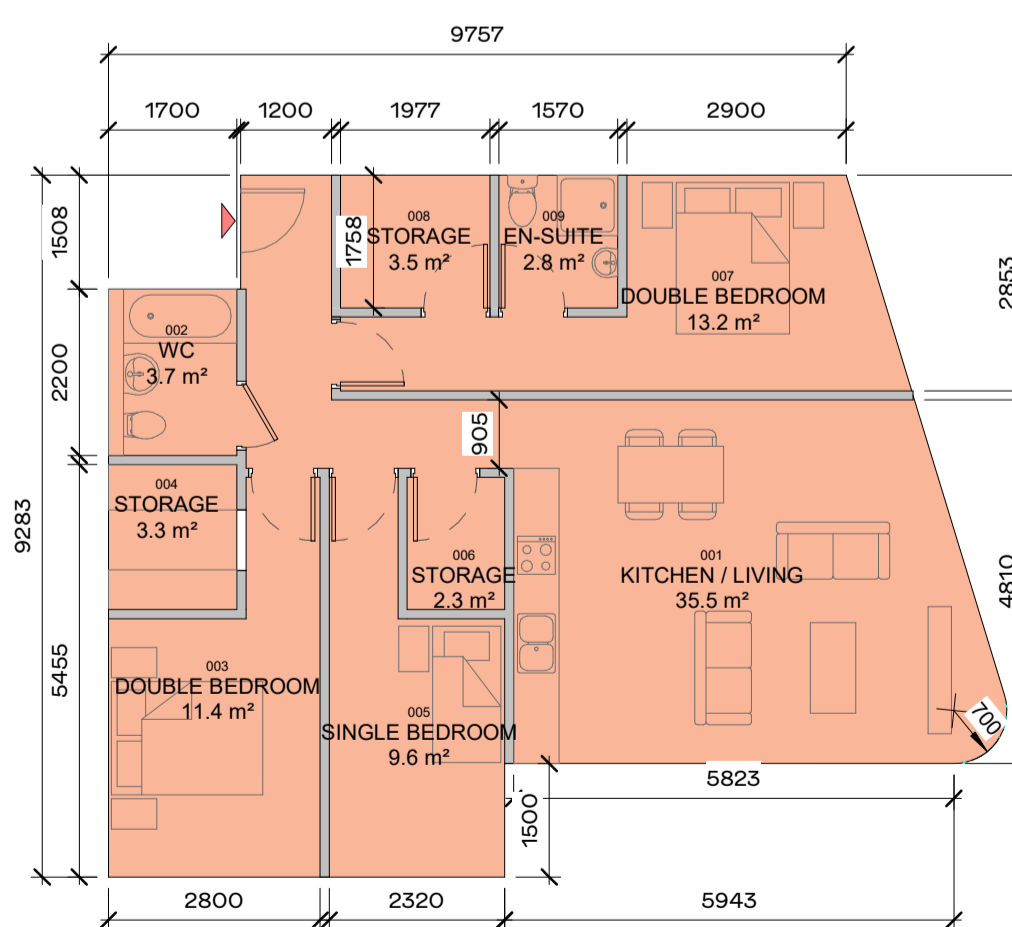
90.2 m 2 6 APARTMENT TYPE - 3B-1A 1:100
