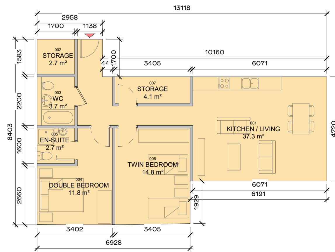
80.6 m 2 1 APARTMENT TYPE - 2B-2A 1:100
