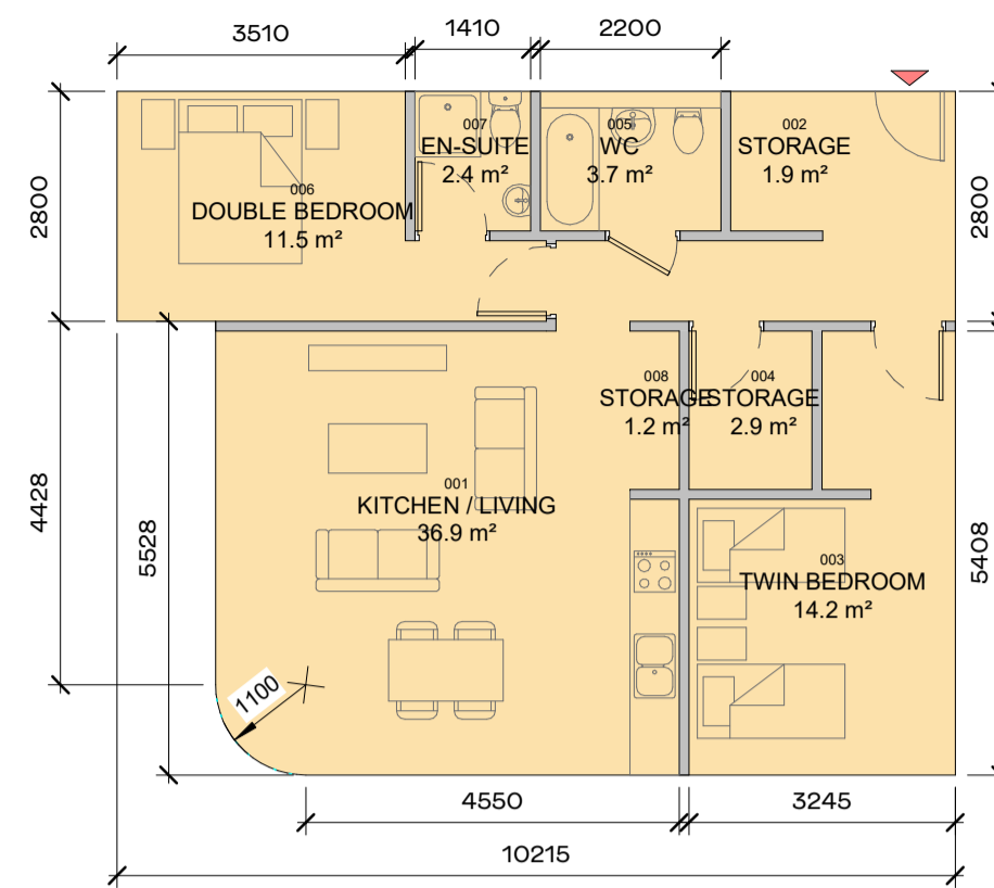
80.3 m 2 2 APARTMENT TYPE - 2B-4A 1:100
