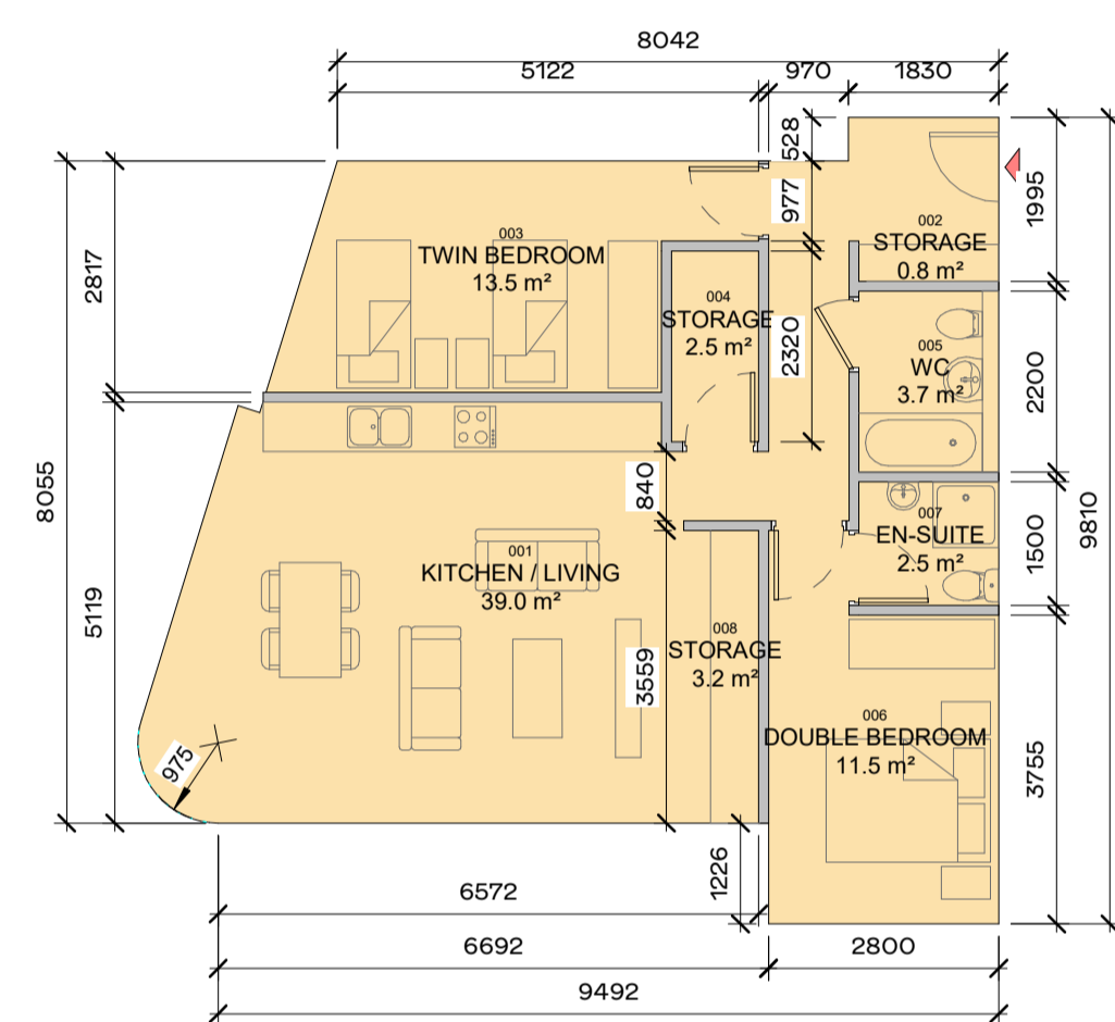
80.3 m 2 3 APARTMENT TYPE - 2B-5A 1:100
